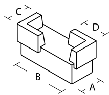
OFFSET BACKRESTS
