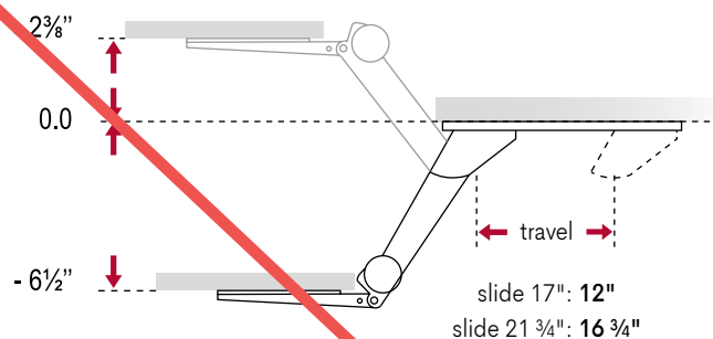
HEIGHT ADJUSTMENT: + 2 3/8" to - 6 1/2"
